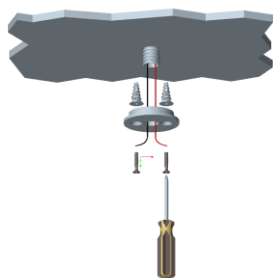
Fix the rosette by screws
